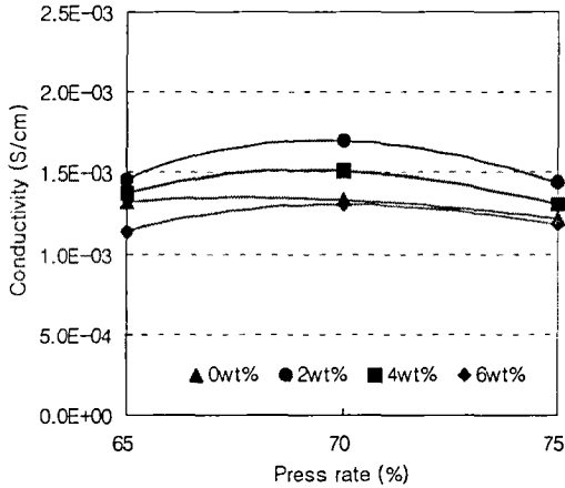
Fig. 4 Conductivity of Anode with different press rate.
