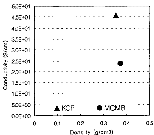
Fig. 3 Electric conductivity of KCF and MCMB
