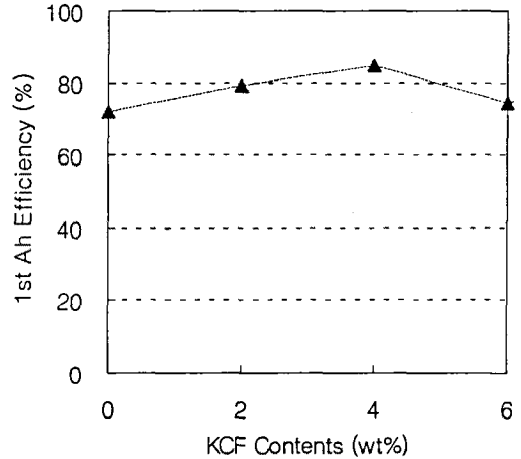
Fig. 6 1st Ah Efficiency of cells with different KCF anode.
