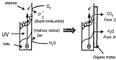
Fig. 1. Schematic diagram for the photocatalytic oxidation decomposition reaction
