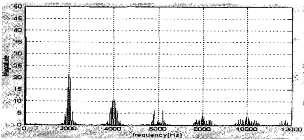
(b)2 phase SVM
