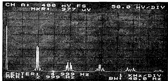
(b)2 phase SVM
