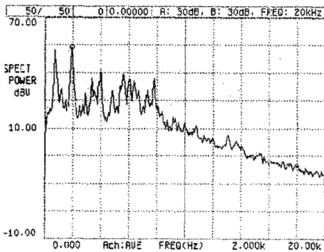
(c) 3 phase SRP-PWM
