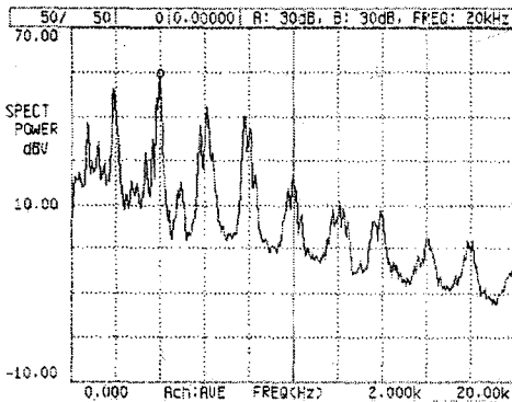
(a) 3 phase SVM
