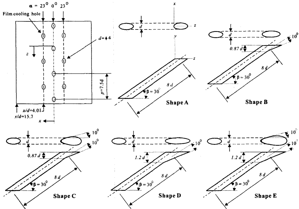
Fig. 1 Overview of showerhead geometries.
