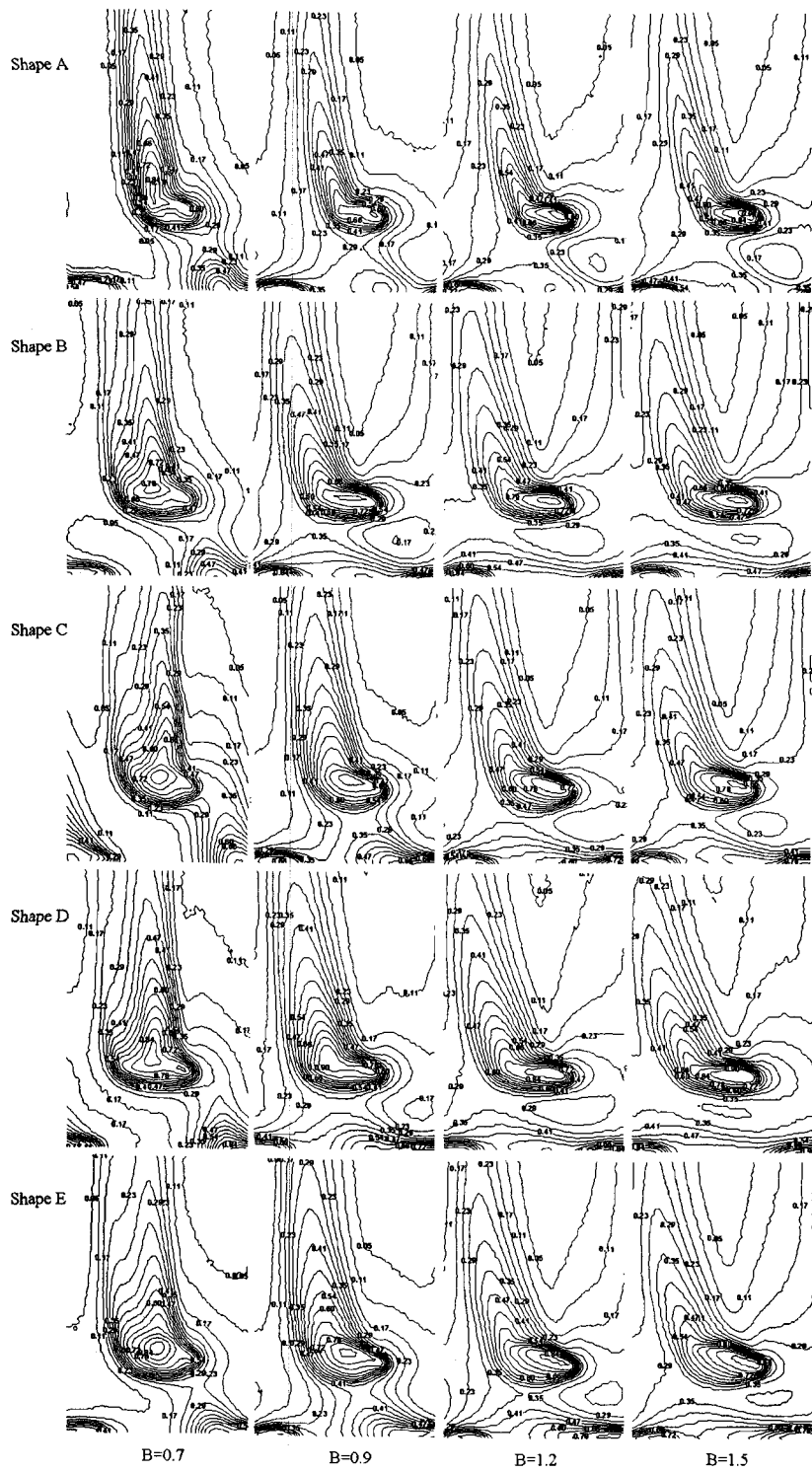
Fig. 2 Film cooling effectiveness distributions at the leading edge surface (measured by IR-camera, 18,700 pixels)
