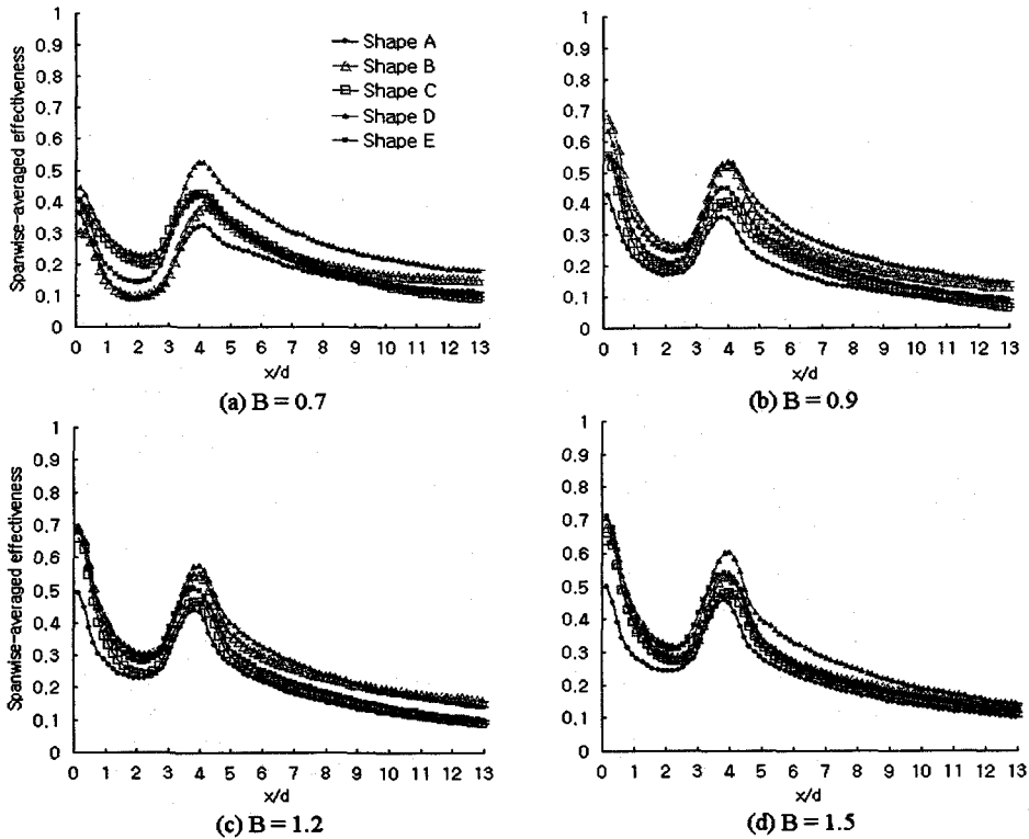
Fig. 3 Spanwise-averaged film cooling effectiveness for different blowing ratios.
