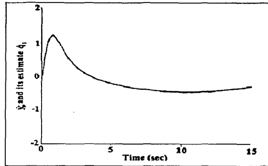
Fig. 3 Estimation of output derivative (Relative degree = 3)
