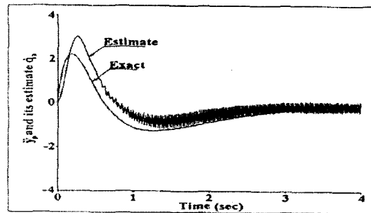
Fig. 4 Estimation of output derivative (Relative degree = 3)
