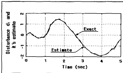
Fig. 2 Disturbance and it's estimation ( Relative degree = 2 )
