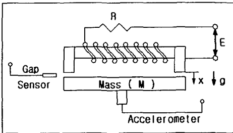
Fig. 2 Electromagnetic Suspension System
