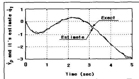
Fig. 1 Estimation of output derivative (Relative degree = 2)
