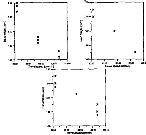
Fig. 5 RMS of travel speed vs. bead geometry (welding current 190A, arc voltage 26V)
