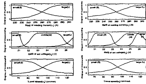
(a) Inferring bead width (b) Inferring bead height
