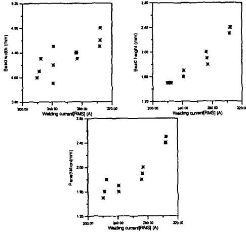
Fig. 3 RMS of welding current vs. bead geometry (arc voltage 26V, travel speed 127.2cm/min)
