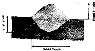
Fig. 1 Bead Geometry
