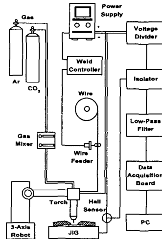
Fig. 2 Schematic diagram of experimental system
