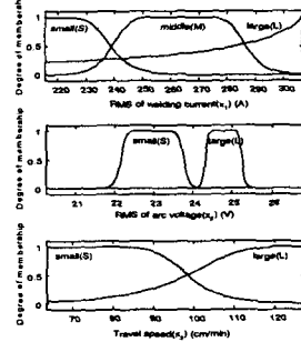
(c) Inferring penetration
