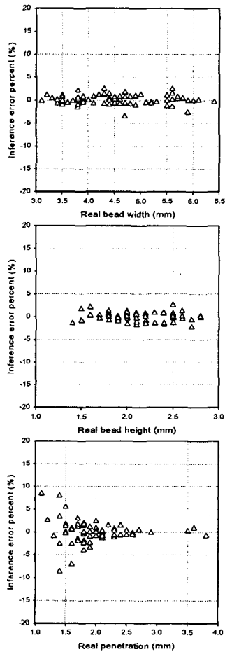
Fig. 7 Inference error percent
