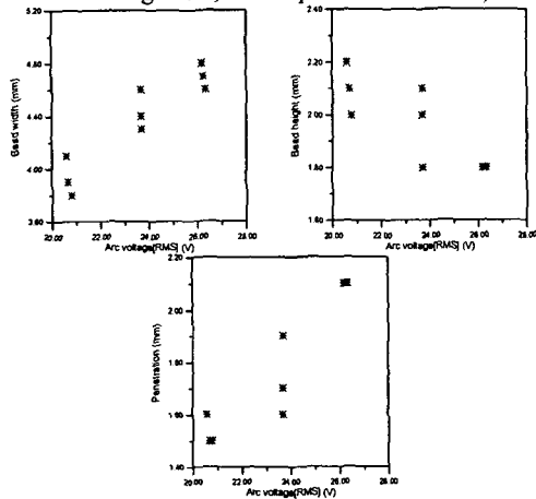
Fig. 4 RMS of arc voltage vs. bead geometry (welding current 190A, travel speed 95.4 cm/min)
