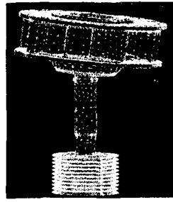
Fig. 7 1st mode shape
