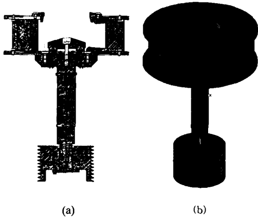
Fig. 2 (a) 2D (b) 3D modeling of Vertical Shaft Impact Crusher rotor
