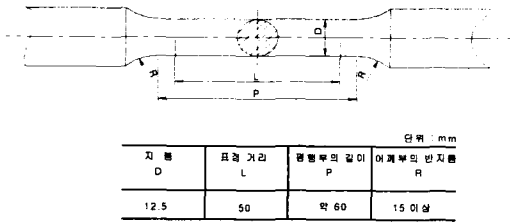
Fig. 1 Configuration of tension specimen
