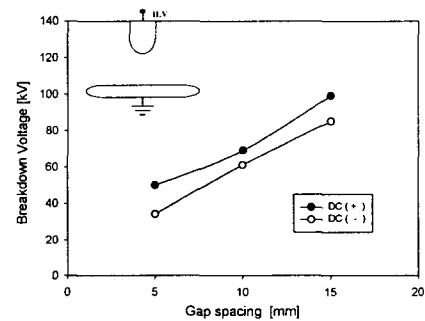
Fig. 5. Surface Flashover Voltage of in in LN 2 (B mode)
