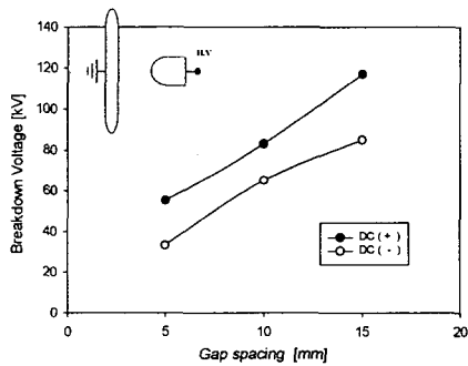
Fig. 3. Surface Flashover Voltage of in in LN 2 (A mode)
