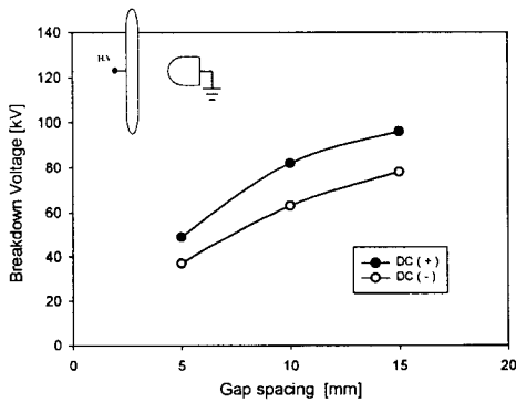
Fig. 7. Surface Flashover Voltage of in LN 2 (C mode)
