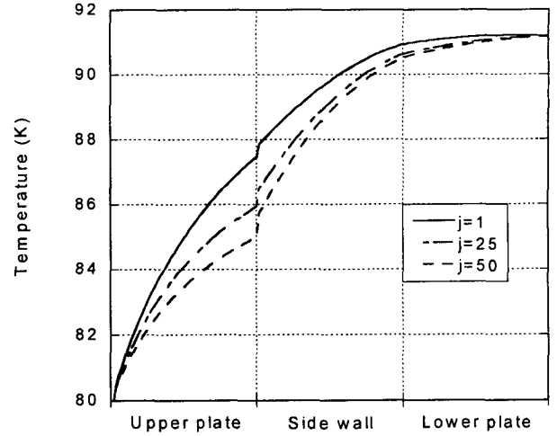
Fig. 4. Temperature distribution in a radiation shield
