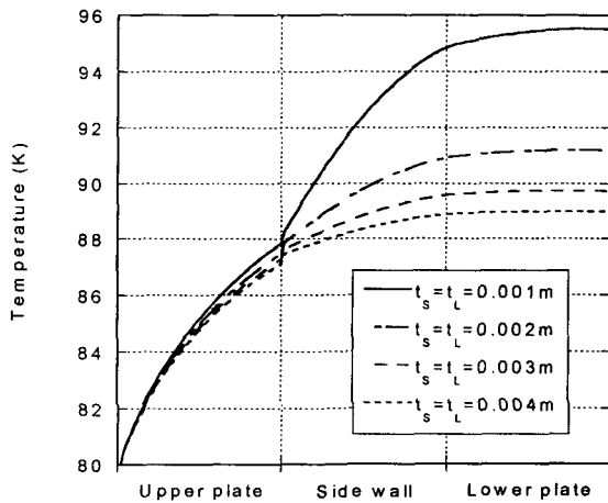
Fig. 6. Effect of thickness of side wall and lower plate on temperature
