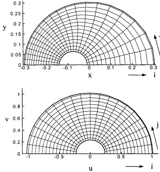
Fig. 3. Physical plane and Numerical plane of upper plate
