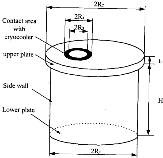
Fig. 1. Schematic diagram of a radiation shield
