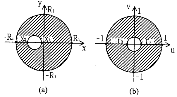
Fig. 2. Conformal mapping by Equation(5)
