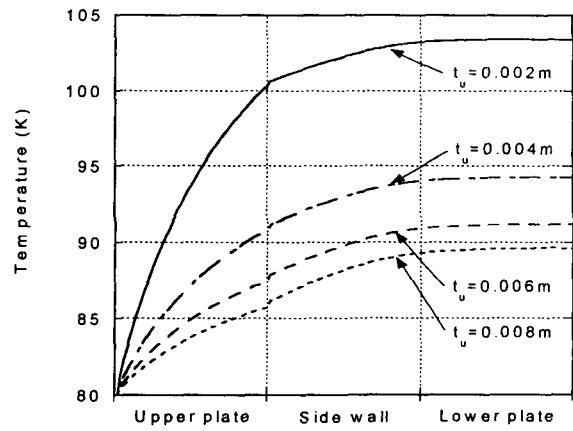
Fig. 7. Effect of thickness of upper wall on temperature
