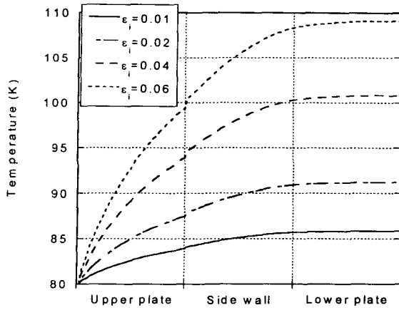
Fig. 5. Effect of emissivity of radiation shield on temperature
