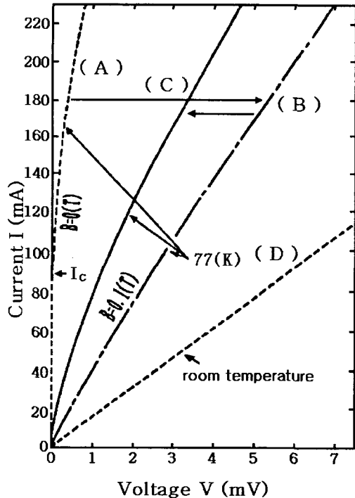
Fig. 1. Current-voltage characteristics of the YBaCuO ceramics.
