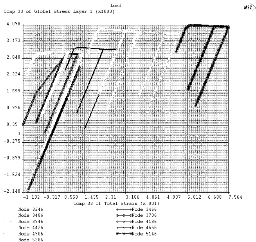
Fig.8 Local behavior of longitudinal stress-strain in case of 0.8\sigma_y - 1.0\sigma_y load condition 1
