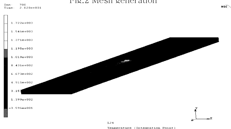
Fig.3 Temperature distribution at 28.28 sec after welding
