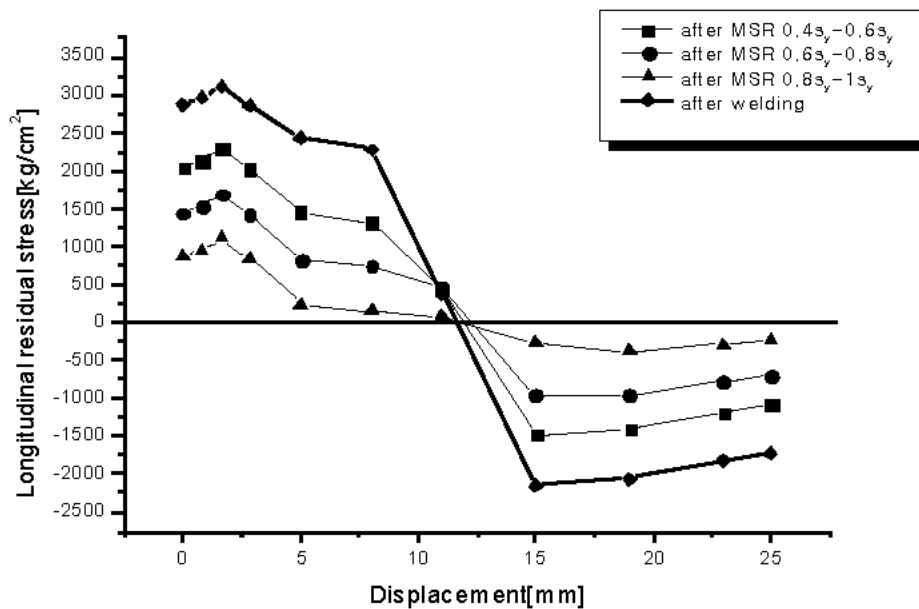
Fig.7 Analysis results for the release of residual stress under variable load conditions
