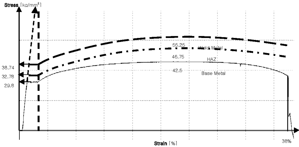
Fig.4 Stress-strain curves of base metal, HAZ, and weld metal
