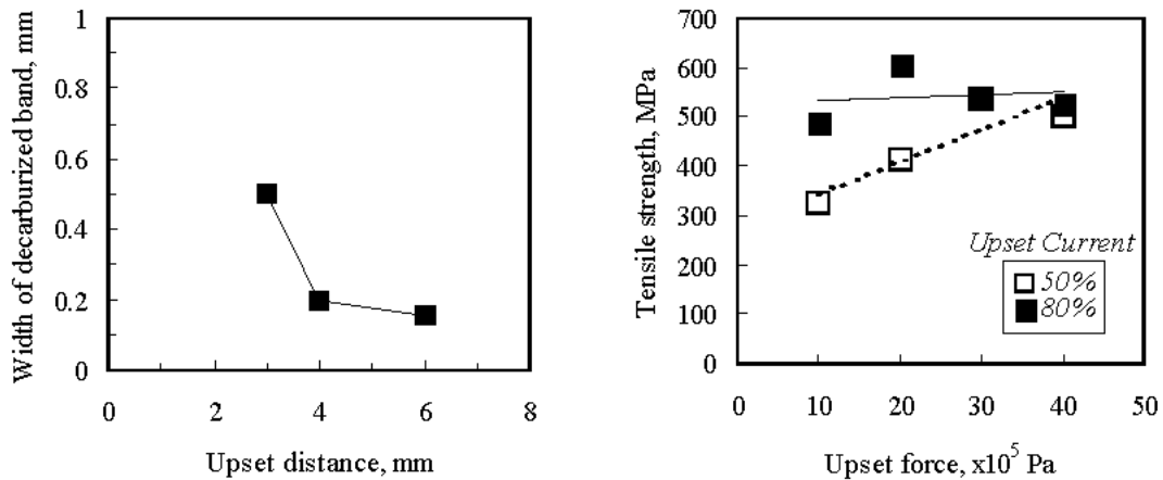
Figure 6. Decarburized band varies with upset distance. Figure 7. Tensile strength as a function of upset force.
