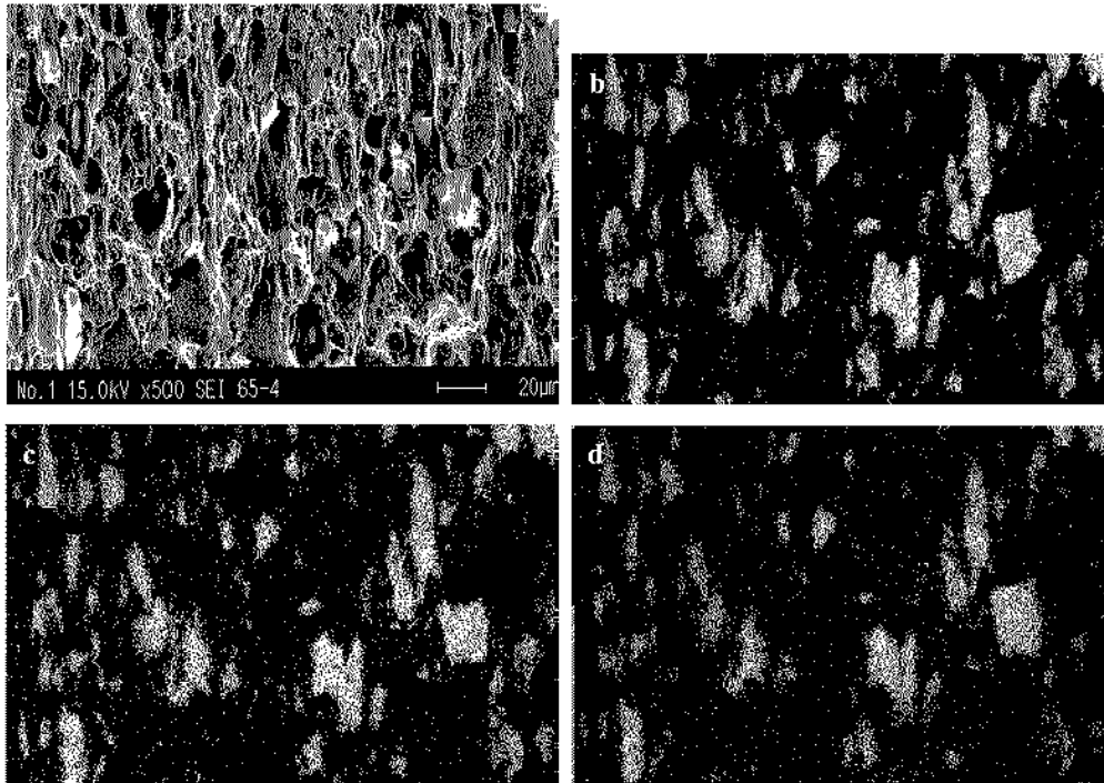
Figure 8. (a) SEM micrograph reveals the element distributions of (b) O, (c) Si, and (d) Mn.
