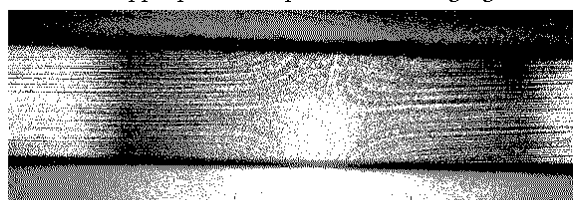
Figure 1. Typical microstructure of flash butt weld showing metal flows.
