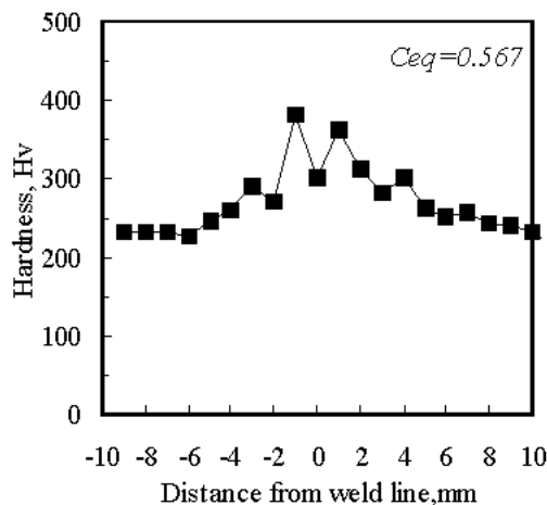
Figure 2. Hardness distribution of a flash butt weld. Figure 3. Maximum hardness as a function of C_{eq} .
