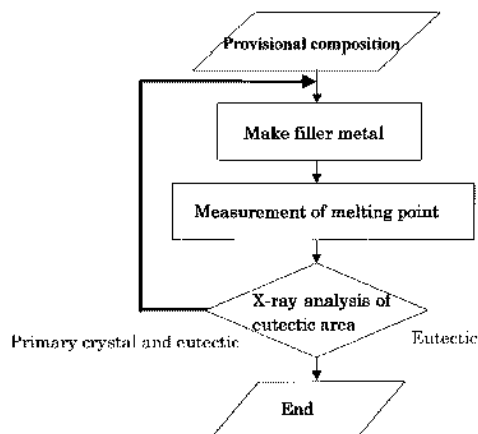
Fig.1 Algorithm of eutectic composition exploration method
