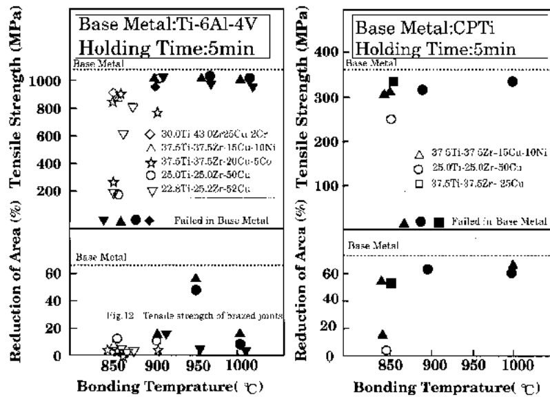
Fig.7 Tensile strength of brazed joints
