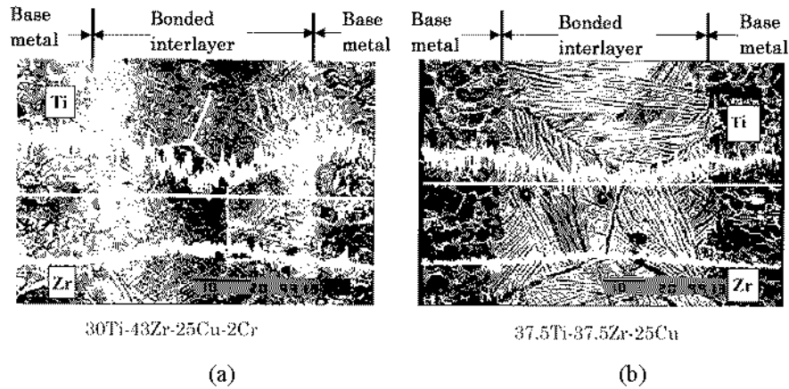
Fig.8 SEM image of bonding interface
