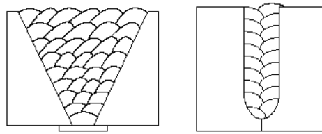
Figure 1. Weld passes of V-shape and narrow gap joint
