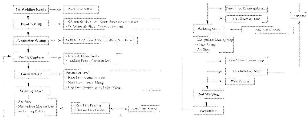
Figure 5. Welding sequence of girth seam welding
