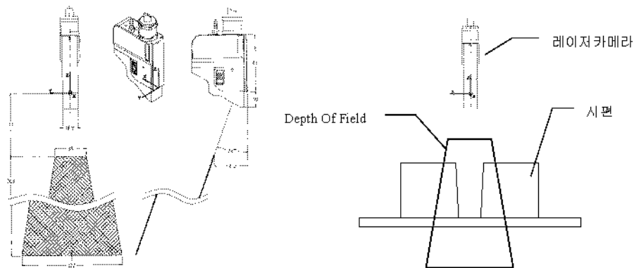
Figure 4. Mini-260 laser vision camera and joint capture
