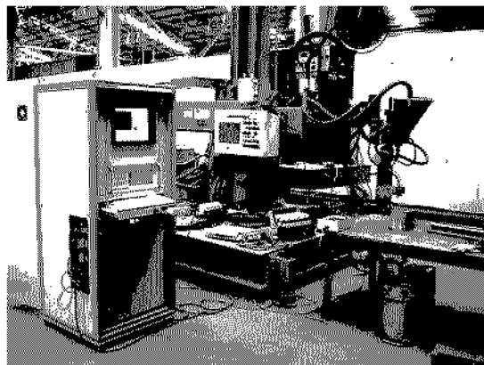
(a) Full automation system (b) Lincoln DC1500 welding power supply
