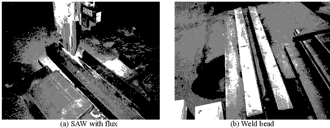
Figure 13. Welding test on the long seam line
