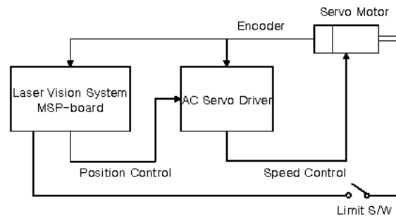
Figure 3. AC servo motor control system
