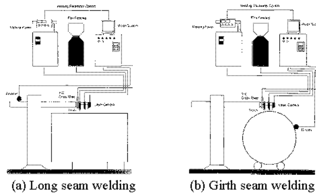
Figure 2. SAW multi-pass welding system
