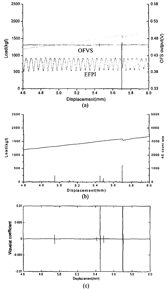
Fig. 3 Load-displacement curve and (a) OFS signal, (b) AE count, (c) WT of OFVS signal during tensile test(4.6-6.0mm).
