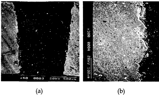
Fig. 9 Cross-Section of ED-Drilled Hole (SEM by (a) X 60 and (b) X 300)
