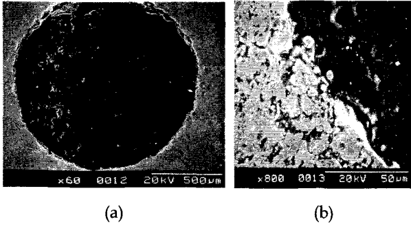
Fig. 8 ED-Drilled Hole (SEM by (a) X 60 and (b) X 800)
