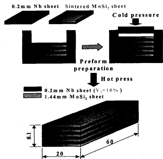
Fig. 1 Fabricating process of Nb/MoSi 2 Laminate Composites.
