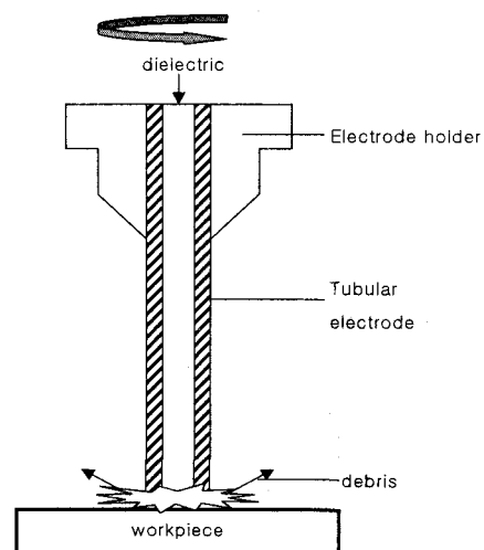
Fig. 3 Schematic diagram for ED-drilling process.
