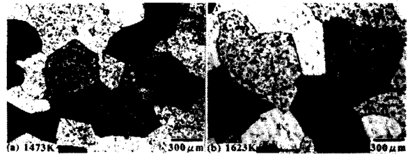
Fig. 5 Optical microscope images of Nb sheet after tempered at different temperatures. (a) 1473K, (b) 1623K
