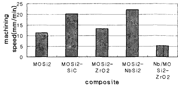
Fig. 10 Machining Speed of Composites
