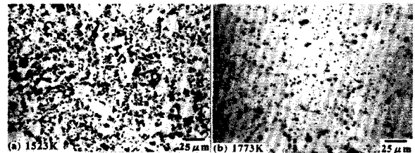
Fig. 4 Optical microscope images of monolithic MoSi 2 materials sintered at different temperatures. (a) 1623K, (b) 1773K
