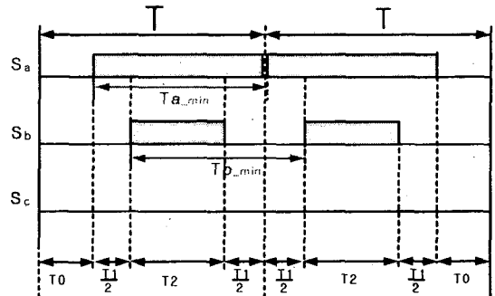
(b) minimum effective switching frequency
