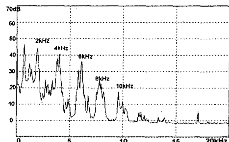
(b) 2 phase SVM
