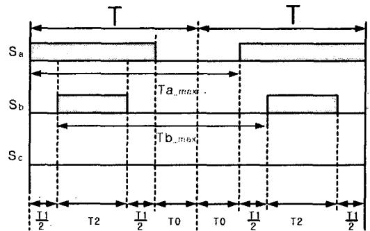
(a) maximum effective switching frequency
