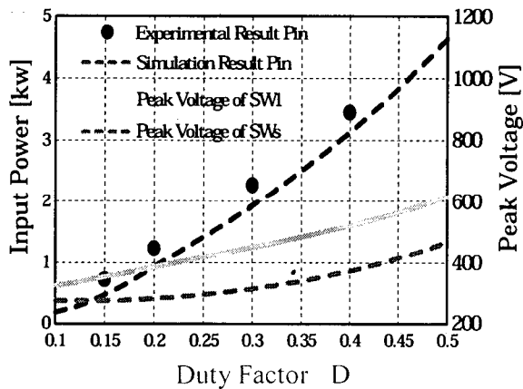
Fig.6 Duty factor vs. input power and peak voltage characteristics
