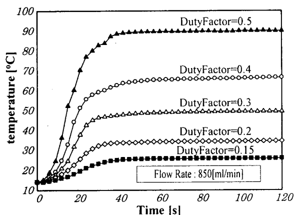
Fig.8 Fluid temperature response characteristics of IH hot water producer and steamer
