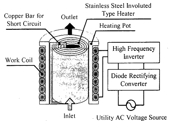
Fig.1 Induction heated hot water producer
