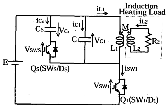
Fig.3 Active voltage clamped edge resonant high-frequency inverter
