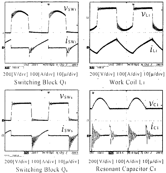
Fig.7 Experimental voltage and current waveforms (Duty Factor D = 0.5 )
