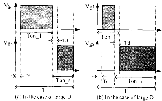
(a) In the case of large D (b) In the case of large D Vg1 : Gate pulse for SW 1 Vgs : Gate pulse for SW s T : One cycle time for high frequency inverter Ton l : Conduction time for SW 1 Ton s : Conduction time for SW s Td : Dead time D : DutyFactor (=Ton l /T)
