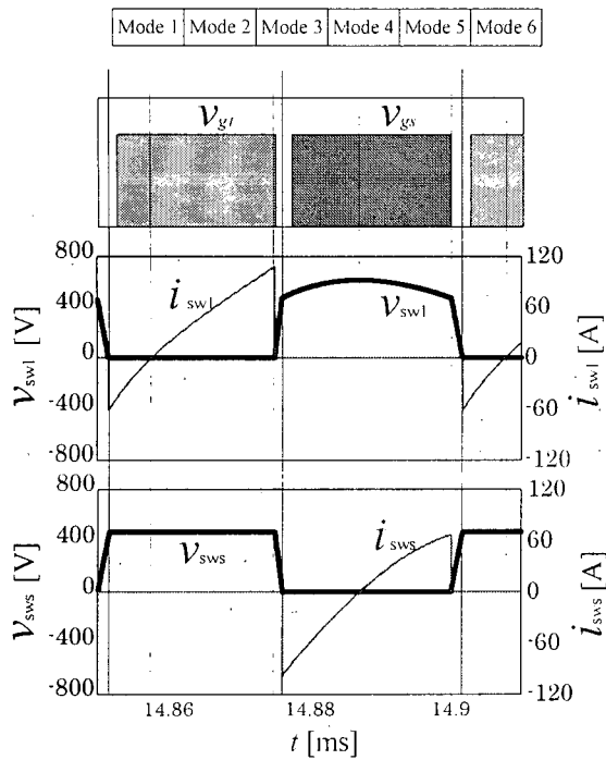
Fig.5 Steady-state switching waveforms
