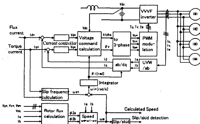
Fig.1 Direct speed calculation method
