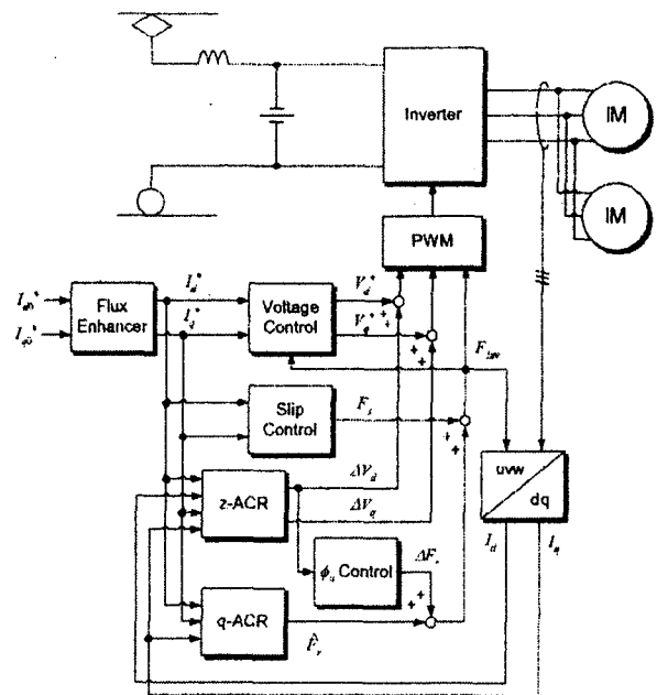
Fig.2 Speed estimation by torque component current feedback
