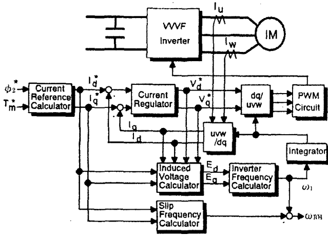
Fig.3 Speed estimation by induced voltage calculation
