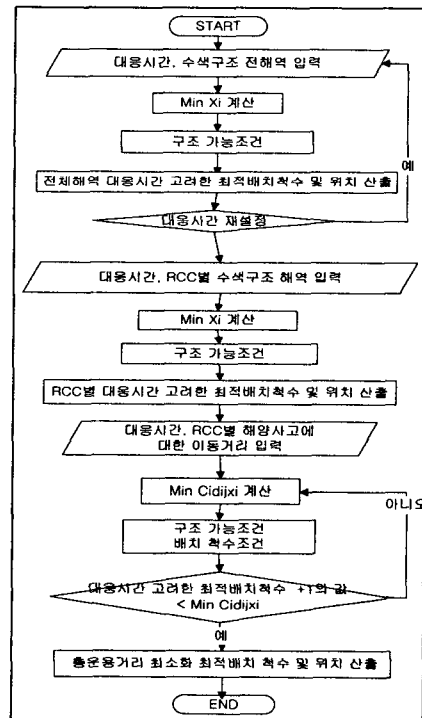
Fig. 3 Flow chart of an optimal allocation model
