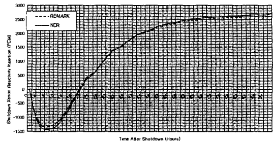
<그림. 7> Comparison of Reactivity Due to Xenon versus Time at BOL (150 MWD/MTU) Following Shutdown after Steady State Operation in REMARK and NDR
