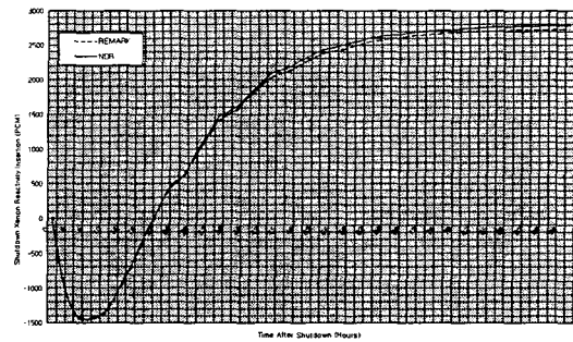
<그림. 8> Comparison of Reactivity Due to Xenon versus Time at MOL (6000MWD/MTU) Following Shutdown after Steady State Operation in REMARK and NDR
