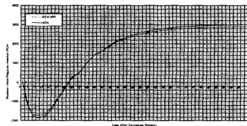
<그림. 9> Comparison of Reactivity Due to Xenon versus Time at EOL (13960 MWD/MTU) Following Shutdown after Steady State Operation in REMARK and NDR
