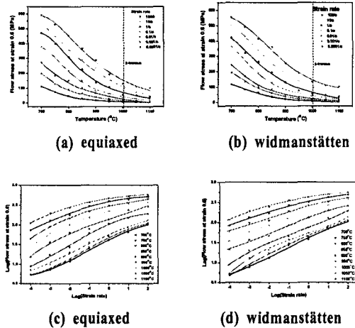
Fig. 5. Variation of flow stress with temperature ((a) and (b)), and with strain rate ((c) and (d)) at a strain of 0.6.
