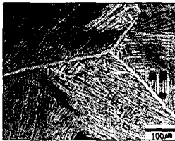
Fig. 2. Optical photograph of widmanstätten microstructure ; heat treated at 1050 °C for 30min and furnace cooling.
