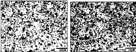
Fig. 1. Optical photographs of as-received microstructure according to the specimen orientation ; (a) longitudinal direction and (b) transverse direction
