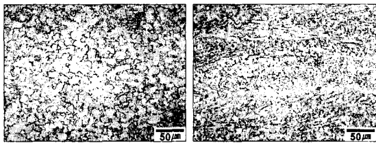
(a) equiaxed 850°C, 10^{-4} /s (b) widmanstätten 850°C, 10^{-4} /s
