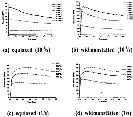
Fig. 3. Flow curve of two microstructures compressed at different temperatures and strain rates..
