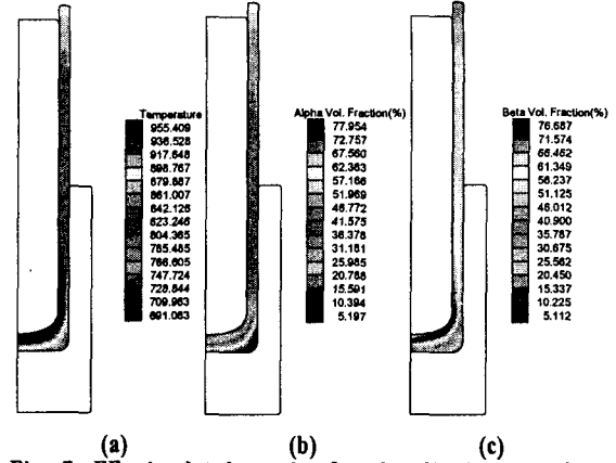
(a) (b) (c) Fig. 7. FE simulated results for the distribution of (a) temperature, (b) volume fraction of \alpha and (c) volume fraction of \beta .
