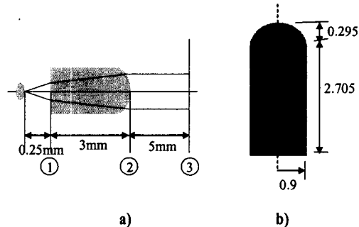
Fig. 1 Design of glass collimating lens, (a) Result of OSLO, (b) Final Design of glass collimating lens
