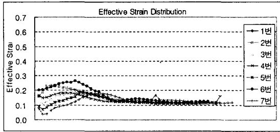
Fig. 4 Effective strain distribution in lens using plat-polished preform
