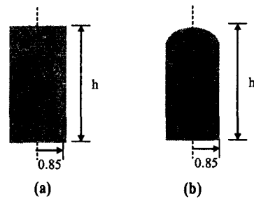
Fig. 3 Design of preform (a) plat-polished preform (b) round-polished preform
