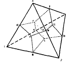
Fig. 1. Tetrahedral finite element and definition of the sub-control volume.
