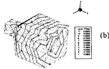
Fig. 4. Predicted filling pattern with respect to time (a) for the complex shaped cavity and (b) for the cavity contracting with an angle.
