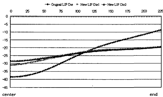
Fig. 8 Distribution of extrusion velocity at the extruded plate
