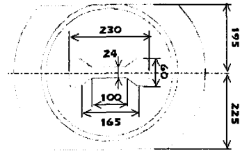
(b) Shape to the inlet of original LIP-die
