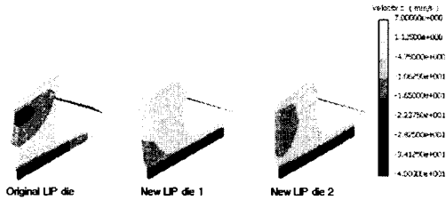
Fig. 7 Result of FE-analysis: Distribution of extrusion velocity
