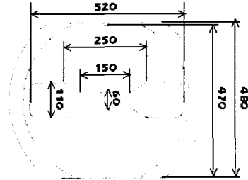
(a) Shape to the outlet of original LIP-die
