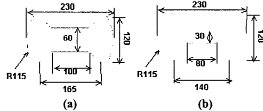
Fig. 5 Shape to the inlet of new LIP-die1, 2(b)
