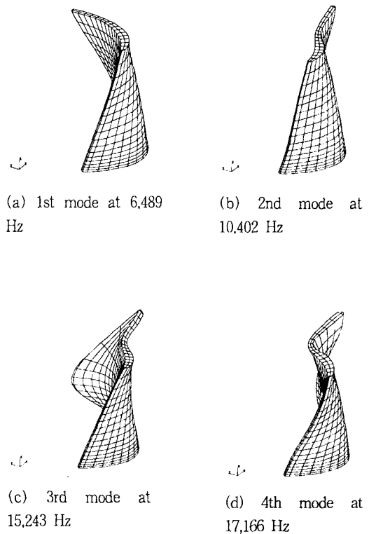
Fig. 5 Mode shapes of the turbine blade
