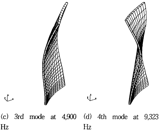
Fig. 4 Mode shapes of the compressor 1st stage blade
