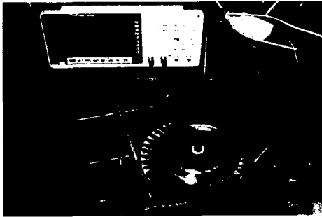
Fig. 7 Impact test set-up for the turbine blade
