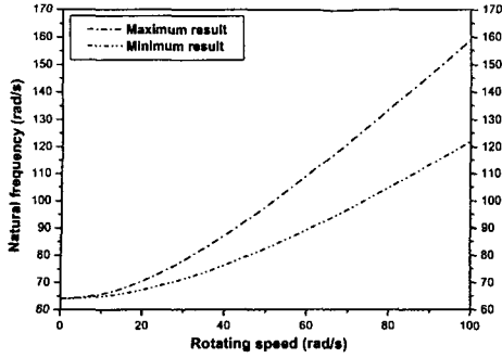
Fig. 6 Band of the 1 st natural frequency versus rotating speed
