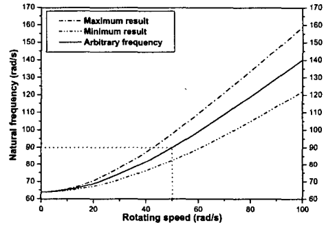
Fig. 9 Specified 1 st natural frequency locus along with the maximum and the minimum loci
