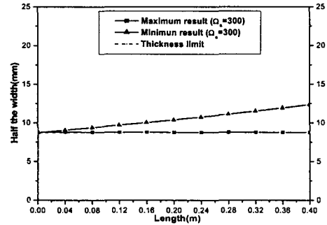
Fig. 5 Half the width shapes which maximize and minimize the 1 st natural frequency
