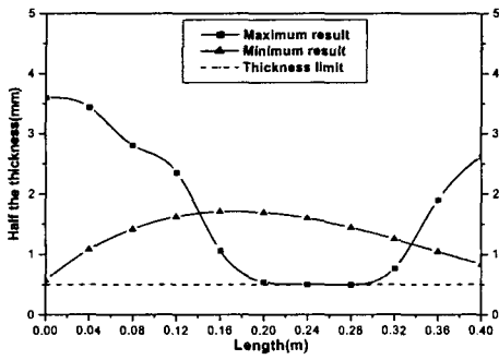
Fig. 7 Half the thickness shapes which maximize and minimize the 1 st natural frequency
