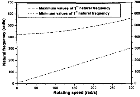
Fig. 2 Band of the first natural frequency versus rotating speed
