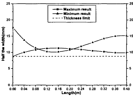
Fig. 8 Half the width shapes which maximize and minimize 1 st natural frequency
