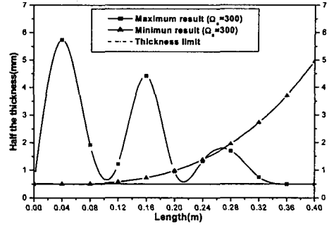
Fig. 4 Half the thickness shapes which maximize and minimize the 1 st natural frequency
