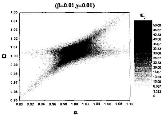
Fig.10 Magnitude of \kappa_2 in \Omega-\alpha plane without angular motion
