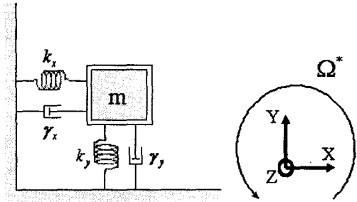
Fig. 3 Modeling of a coupled microgyroscope
