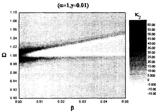
Fig.9 Difference of \kappa_2 between angular motion output ( \delta = 0.01 ) and no angular motion output ( \delta = 0 ) in \Omega-\beta plane
