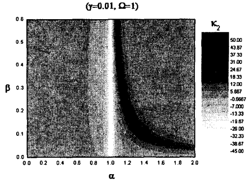
Fig.7 Difference of \kappa_2 between angular motion output ( \delta = 0.1 ) and no angular motion output ( \delta = 0 ) in \alpha - \beta plane
