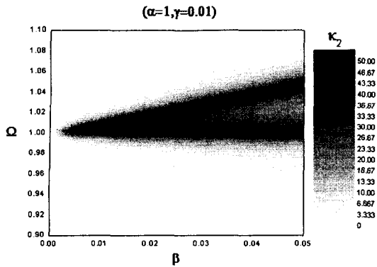
Fig.8 Magnitude of \kappa_2 in \Omega-\beta plane without angular motion
