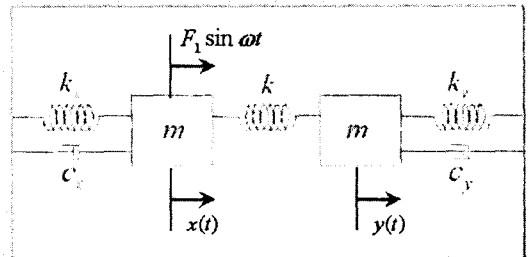
Fig.4 Simplified Modeling of a coupled structure
