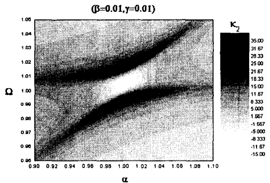
Fig.11 Difference of \kappa_2 between angular motion output ( \delta = 0.01 ) and no angular motion output ( \delta = 0 ) in \Omega-\alpha plane
