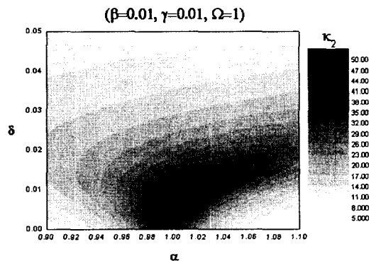
Fig.12 Magnitude of \kappa_2 in \alpha-\delta plane
