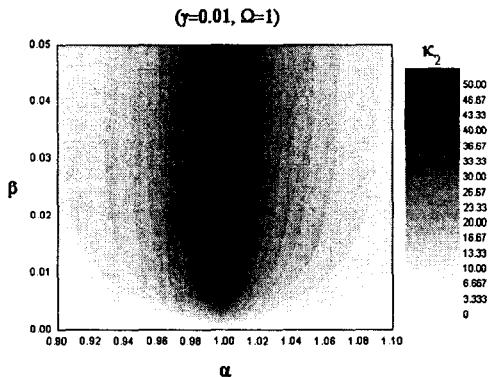
Fig.5 Magnitude of \kappa_2 in \alpha - \beta plane without angular motion
