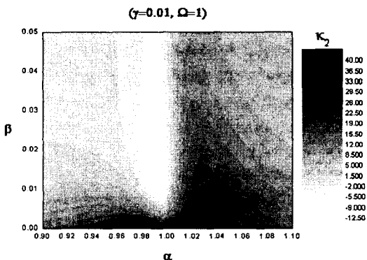
Fig.6 Difference of \kappa_2 between angular motion output ( \delta = 0.01 ) and no angular motion output ( \delta = 0 ) in \alpha - \beta plane
