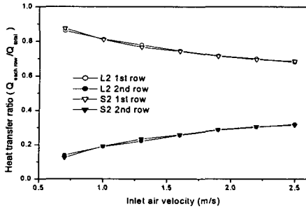
Fig 4 Contribution of individual rows to total heat transfer
