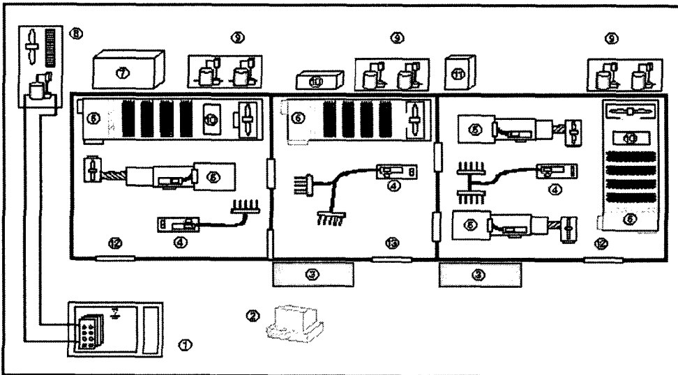
①Water bath ②Data acquisition system ③Control panel ④Sampling unit ⑤Code tester ⑥Air conditioner ⑦Power supply ⑧Cooling tower ⑨Refrigerator ⑩Humidifier ⑪Frequency transfer device ⑫Indoor room ⑬Outdoor room
