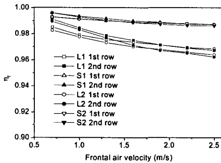
Fig 5 Fin efficiency of heat exchangers
