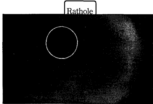
Fig. 8 Ratholes in the hopper without water supply
