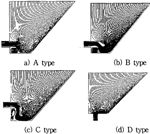
Fig. 4 Stream line at the different hopper types
