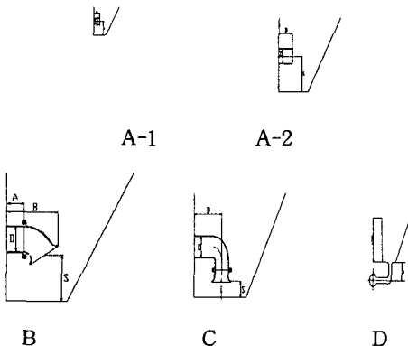
Fig. 3 Entrances of the sludge discharge pipe
