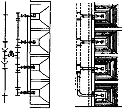
(a) Integration line (b) Single line Fig. 2 Forms of the sludge discharge line
