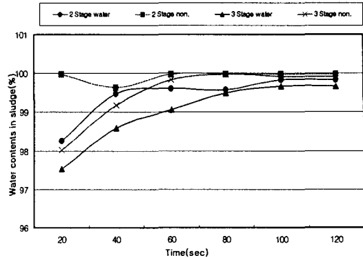
Fig. 10 Water contents in sludge with and without water supply nozzle
