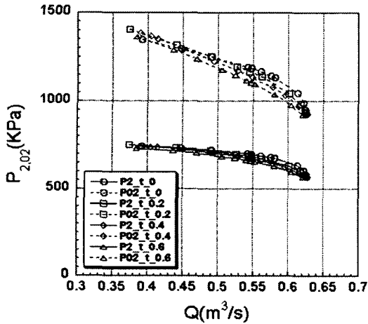
Fig. 5 Comparison of pressure at impeller outlet
