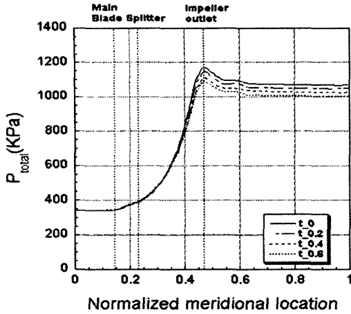
Fig. 9 Variation of total-to-total pressure along the flow passage
