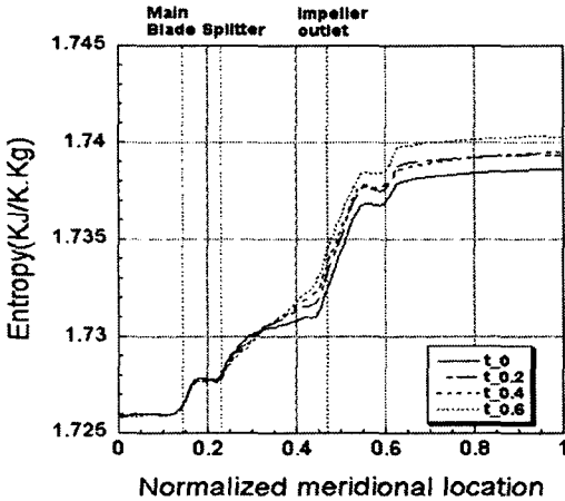
Fig. 10 Variation of entropy along the flow passage
