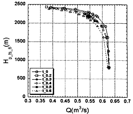
Fig. 7 Comparison of polytropic head at VLD outlet(6)
