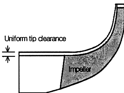
Fig. 1 Tip clearance uniformly distributed from the leading to trailing edge of the impeller
