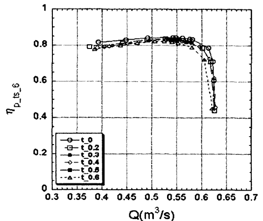
Fig. 8 Comparison of polytropic efficiency at VLD outlet(6)
