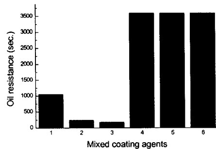
Fig. 2. Oil resistance of paperboard after coating with mixed coating agents.
