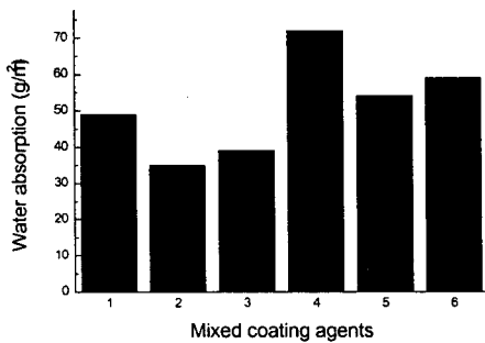
Fig. 1. Water absorption of paperboard after coating with mixed coating agents.
