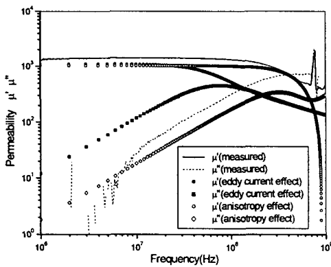
Fig. 5. Permeability vs. frequency for the Co_{87.56}Nb_{6.45}Zr_{1.65}Pd_{4.34}
