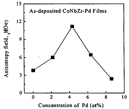
Fig. 4. Change in the anisotropy field as a function of amount of Pd added in the amorphous CoNbZr films.
