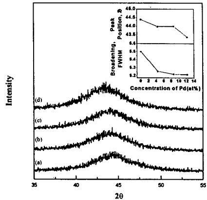
Fig. 2. X-ray diffraction patterns of as-deposited CoNbZr-Pd films
