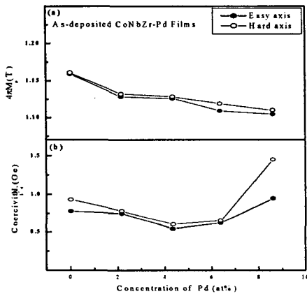
Fig. 3. Changes in the saturation magnetization (a) and the coercivity (b) as a function of amount of Pd addition for amorphous CoNbZr films
