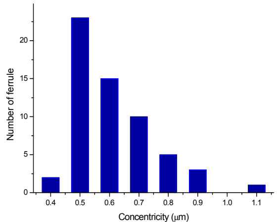
Fig. 5 Concentricity distribution of Ferrule
