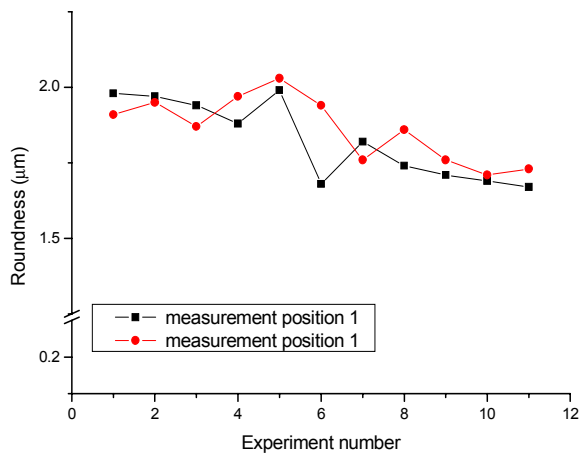
Fig. 6 Roundness of ferrule
