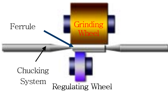
Fig. 4 Processing concept of ferrule grinding
