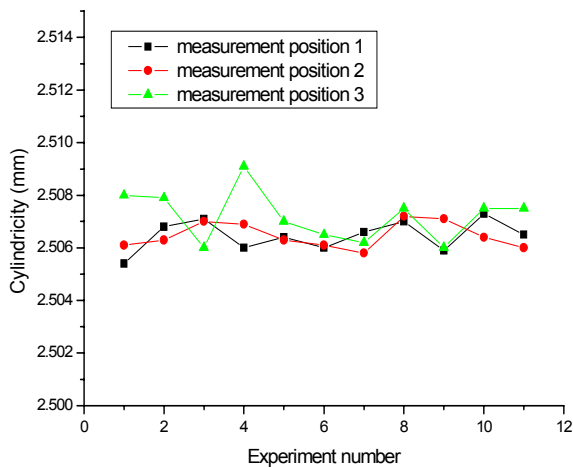
Fig. 7 Cylindricity of ferrule
