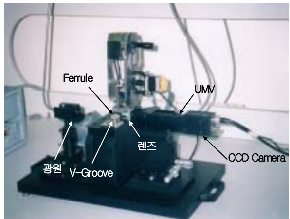
Fig. 3 Concentricity measurement device
