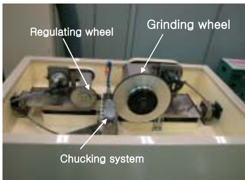
Fig. 1 Photograph of co-axle grinding machine
