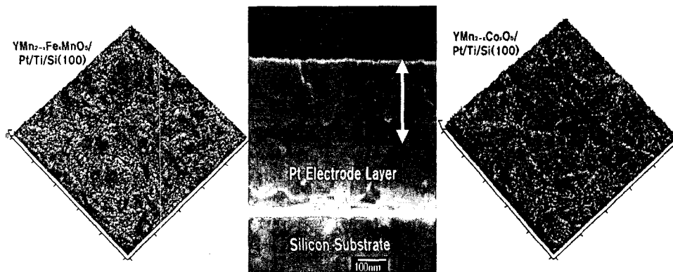
Fig. 1. Atomic force microscopy(AFM) and FE-SEM images of sol-gel derived polycrystalline Y\text{Mn}_{2-x}(\text{Fe,Co})_x\text{O}_{5-\delta} thin films.
