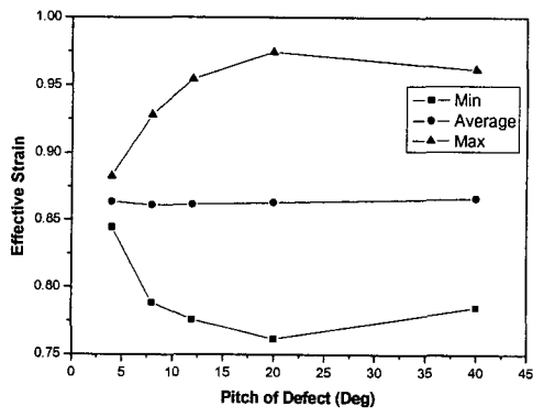
Fig. 3.3 Effective strain of model using 90 elements in circumferential direction with respect to pitch of defects
