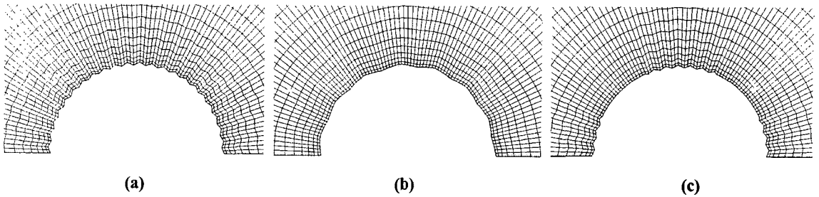
Fig. 2.3 Modeling of defects:(a) defect with 8 mm depth and 4° pitch; (b) defect with 8 mm depth and 12° pitch; (c) defect with 8 mm depth, 4° pitch and 45° interval
