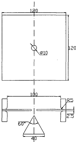
Fig. 2.1 Hole expansion test specimen and tooling
