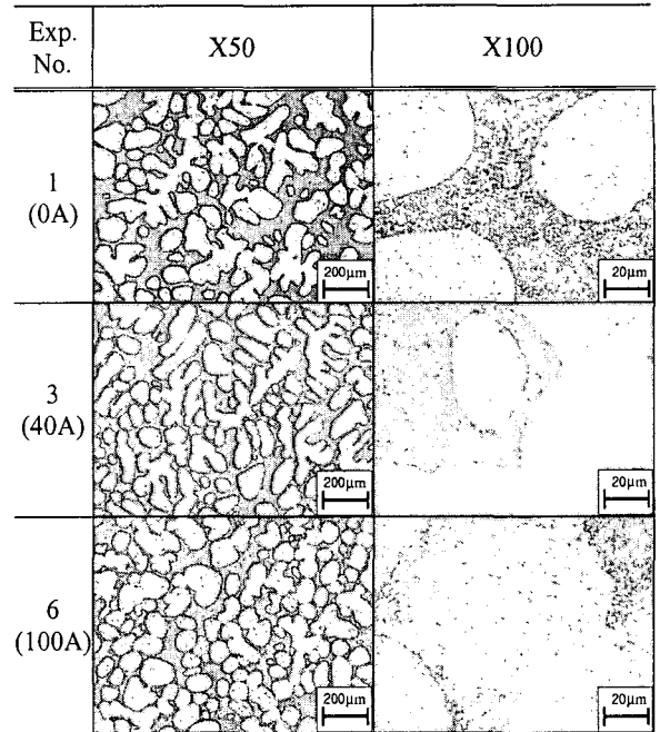
Fig. 4 The comparison of microstructure among experimental conditions.
