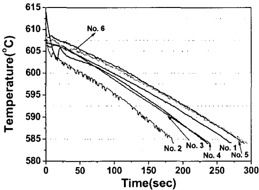
Fig. 3 The temperature profiles at each experimental condition during electromagnetic stirring.
