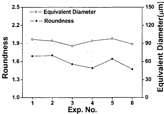
Fig. 7 The comparison of mean roundness and mean equivalent diameter at each experimental condition.
