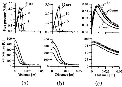
Fig. 3: The effects of frequencies, wall thicknesses and reinforcements: (a) f=18 GHz, (b) 10.6 GHz with P=1.1 MW/m 2 , and (c) f=18 GHz, (b) 10.6 GHz with P=1.1 kW/m 2 .
