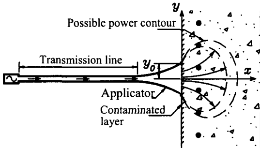
Fig. 1: Sketch of microwave power decontamination system.
