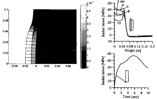
Fig. 4: The strain and stress contour of the concrete wall exposed to 10 sec microwave heating with f=18 GHz and P_0=1.1 MW/m 2 .
