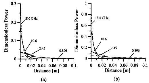
Fig. 2: Examples of volumetric heat generations with (a) the full reflection at the surface of the concrete wall and (b) no reflection. Here, reinforcing bars are located 2.5 cm under the surface to which waves are incident.
