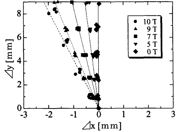
Fig. 10 Path of O_2 bubble under water as a parameter of magnetic field ( x = -1 cm, V = 12\text{--}16 mm 3 )
