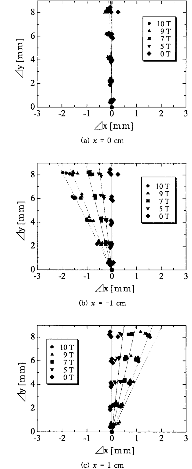
Fig. 8 Path of \text{O}_2 bubble under water as a parameter of magnetic field ( V = 29\text{--}33 \text{ mm}^3 )
