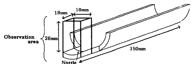
Fig. 6 Illustration of the sample cell
