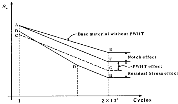
Fig. 1 Effect of residual stress and notch
