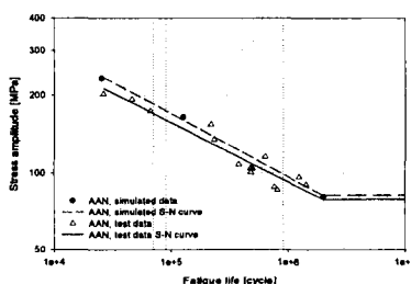
Fig. 2 Test and simulation; as-welded specimens
