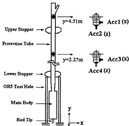
Fig. 1 Schematic view of the fuel capsule
