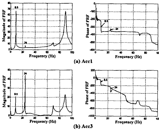
Fig. 3 FRF and phase angle of the fuel capsule in air in the x direction
