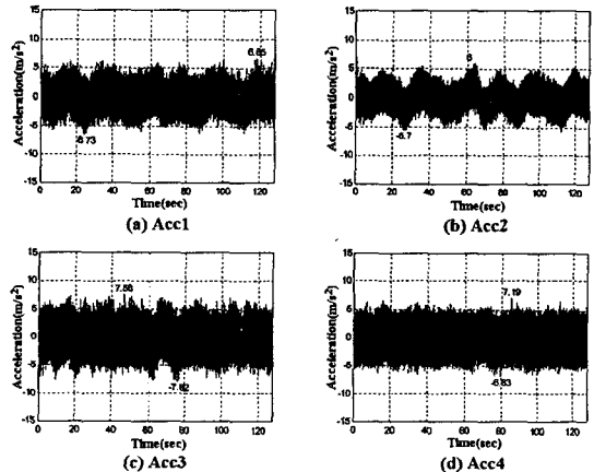
Fig. 6 Acceleration time history of the fuel capsule for the 100% flow
