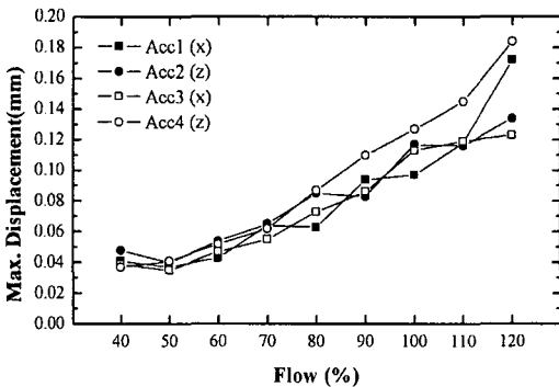
Fig. 8 Max. displacement of the fuel capsule with flow
