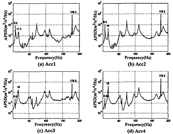
Fig. 9 Auto power spectrum density function of the fuel capsule at 100% flow in the x direction
