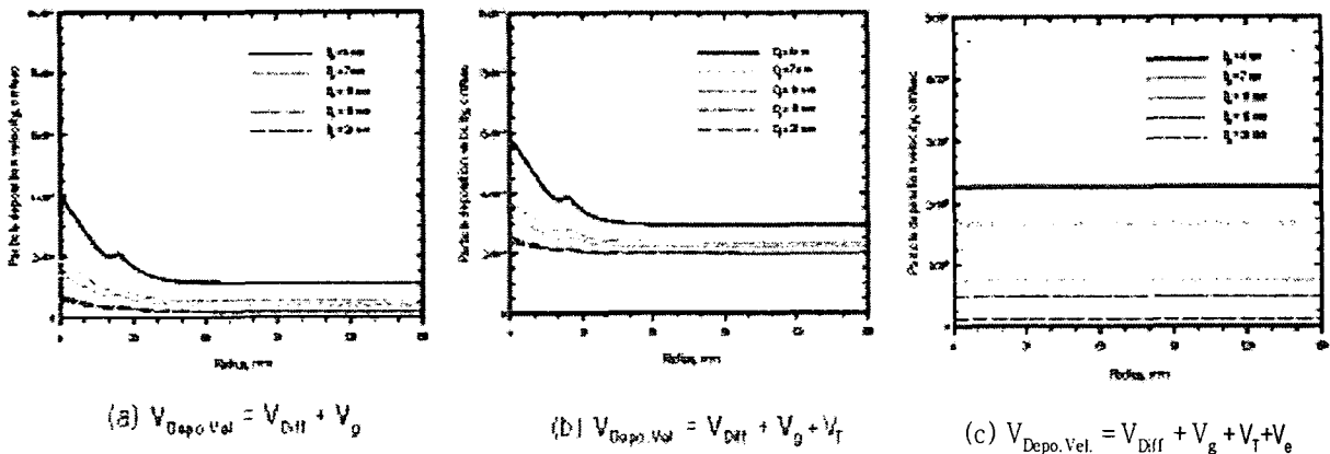
Fig. 3 Particle deposition velocity with respect to radius of wafer according to particle deposition mechanism ( Q_{in} = 3 \text{ lpm} ).
