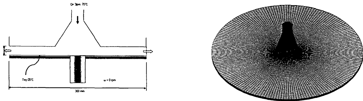
Fig. 1 Schematic diagram of nanoparticle chamber and calculation mesh.
