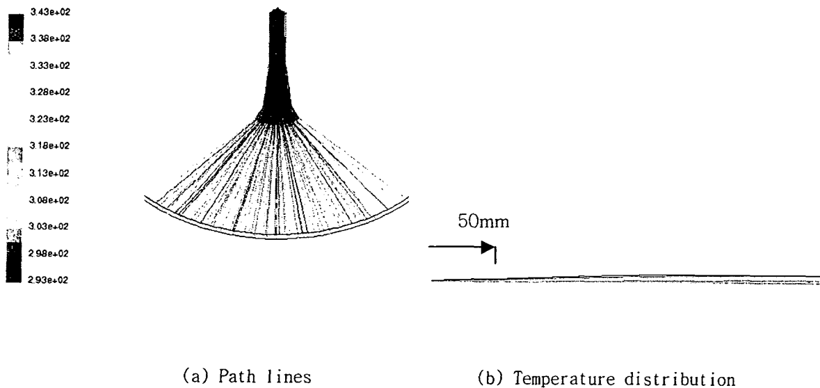
Fig. 2 Fluid path lines and temperature distribution in the chamber.
