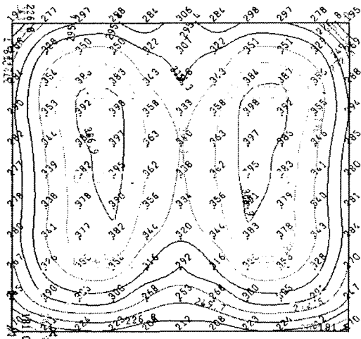
Fig. 2. Iso-lux diagram of grid by simulation of sy
