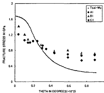
Fig. 3 Theoretical and Experimental Data for Fracture Strength of Graphite/Epoxy by Tsai & Wu and Lagace[5]
