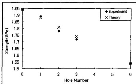
Fig. 6 Experimental and Theoretical Fracture Strength Graph
