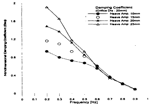
Fig. 6: Variation of non-dimensional damping coefficient with Frequency (orifice dia.=20mm)
