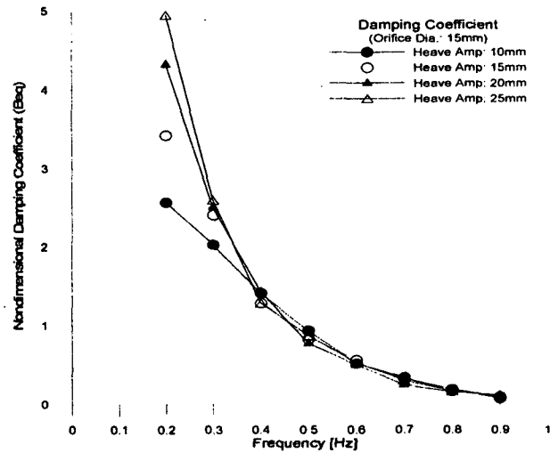
Fig. 5: Variation of non-dimensional damping coefficient with frequency (orifice dia.=15mm)
