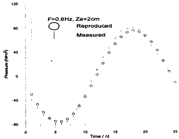
Fig. 19: Comparison of measured pressure with reproduced pressure ( F=0.8\text{Hz} , Z_a=2\text{cm} )
