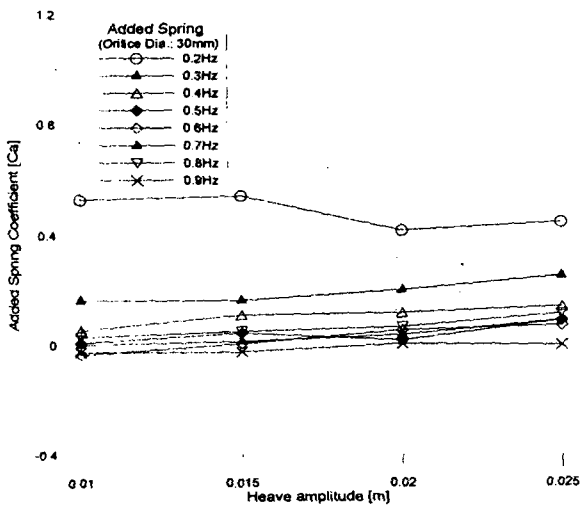
Fig. 17: Variation of non-dimensional added spring coefficient with heave amplitude (orifice dia.=30mm)
