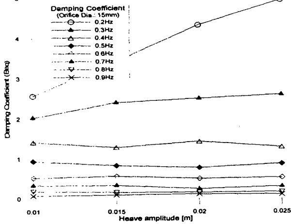
Fig. 8: Variation of non-dimensional damping coefficient with heave amplitude (orifice dia.=15mm)
