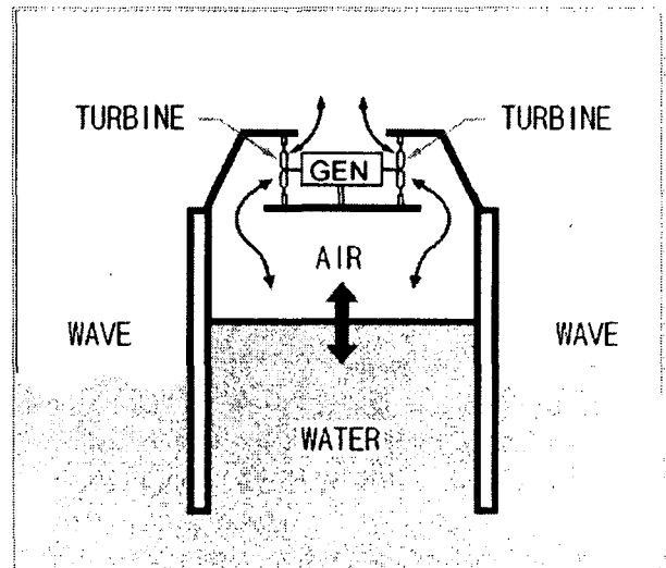
Fig. 1: Concept of OWC Type Wave Energy Absorption
