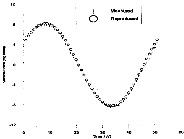
Fig. 4 : Comparison of measured heave force with reproduced force (frequency = 0.4Hz, z_a = 2 cm)
