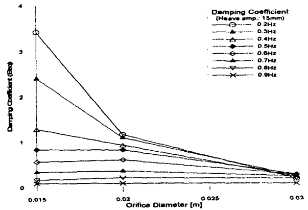
Fig. 11 : Variation of non-dimensional damping coefficient with orifice diameter ( Z_a = 1.5cm )
