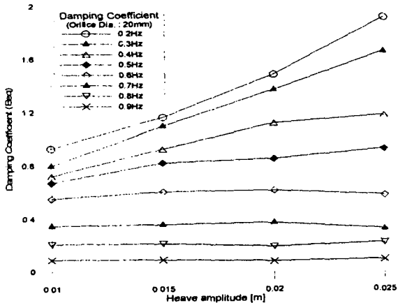
Fig. 9: Variation of non-dimensional damping coefficient with heave amplitude (orifice dia.=20mm)
