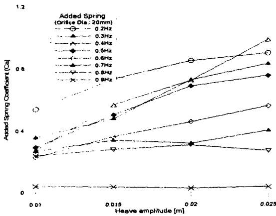
Fig. 16: Variation of non-dimensional added spring coefficient with heave amplitude (orifice dia.=20mm)
