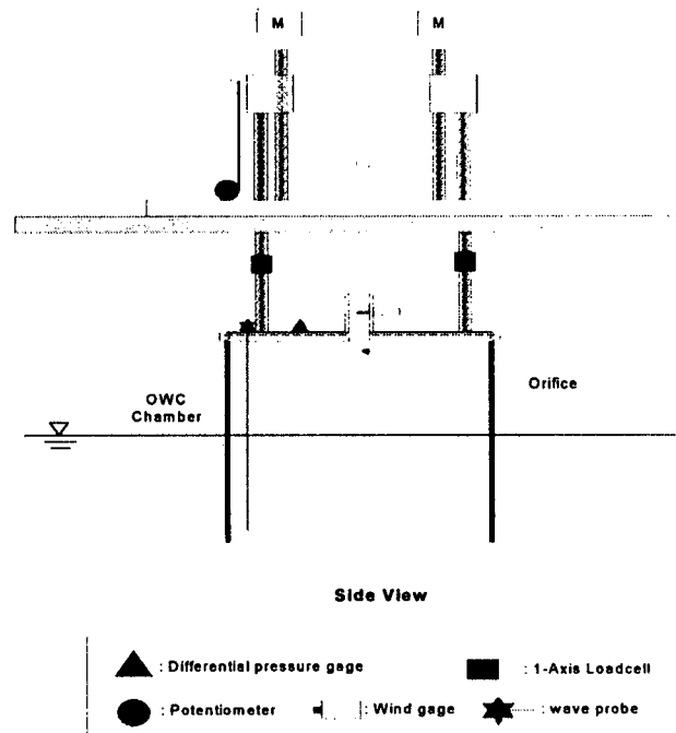
Fig. 2: Measuring System
