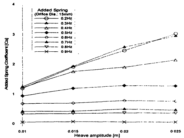
Fig. 15: Variation of non-dimensional added spring coefficient with heave amplitude (orifice dia.=15mm)
