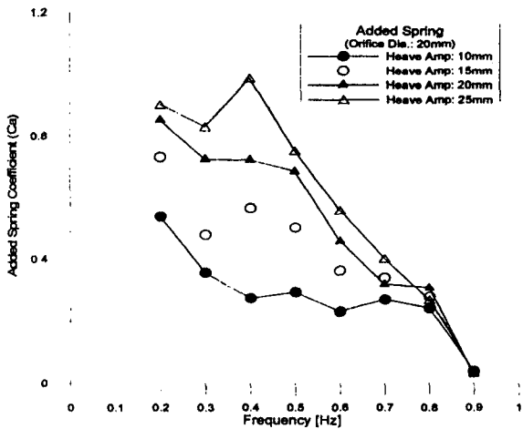
Fig. 13: Variation of non-dimensional added spring coefficient with frequency ( orifice dia.=20mm)
