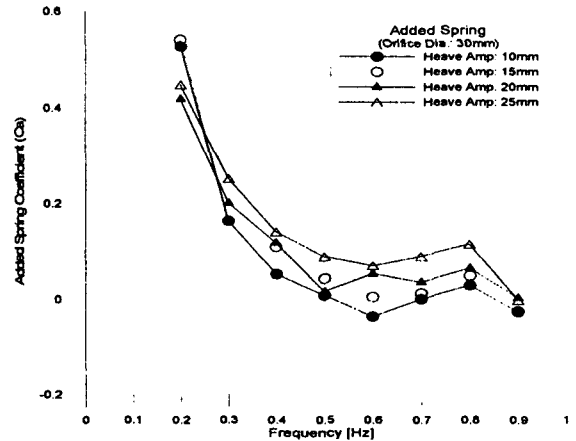
Fig. 14: Variation of non-dimensional added spring coefficient with frequency (orifice dia.= 30mm)
