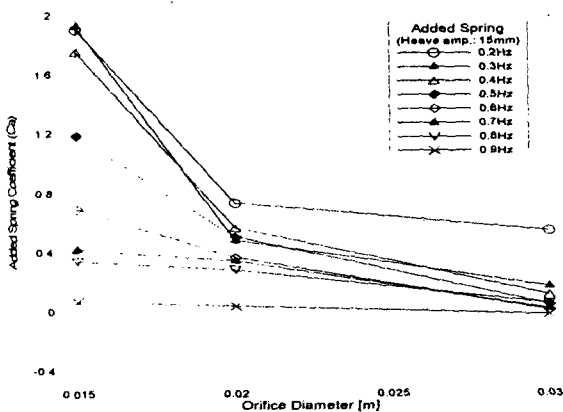
Fig. 18: Variation of non-dimensional added spring coefficient with orifice diameter ( Z_a = 1.5\text{cm} )
