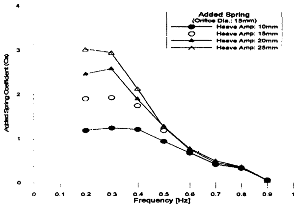
Fig. 12: Variation of non-dimensional added spring coefficient with frequency (orifice dia.=15mm)
