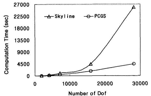
Fig. 6 Time comparison for lid-driven flow (cubic elements, Re = 1000 )
