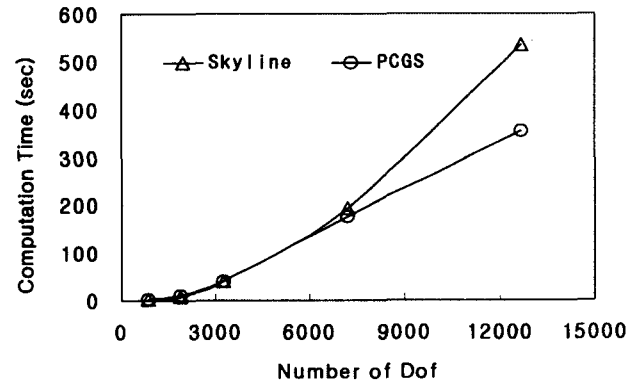
Fig. 5 Time comparison for lid-driven flow (quadratic elements, Re = 1000 )
