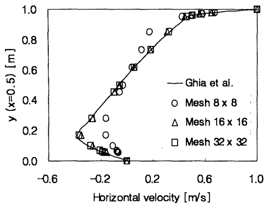
Fig. 7 A comparison of velocity solutions with Ghia, Ghia and Shin(1982)
