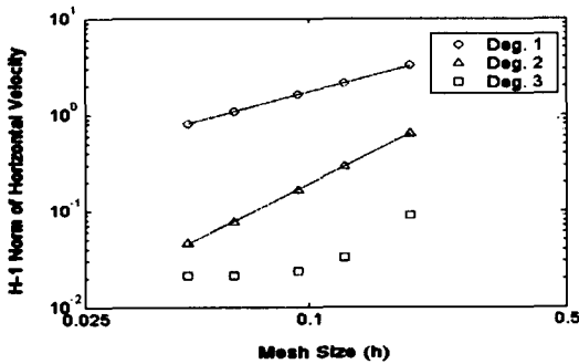
Fig. 2 Convergence trend for Kovaszny flow
