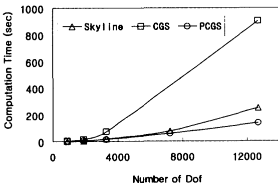
Fig. 3 Time comparison for Kovaszny flow (quadratic elements, Re = 40 )
