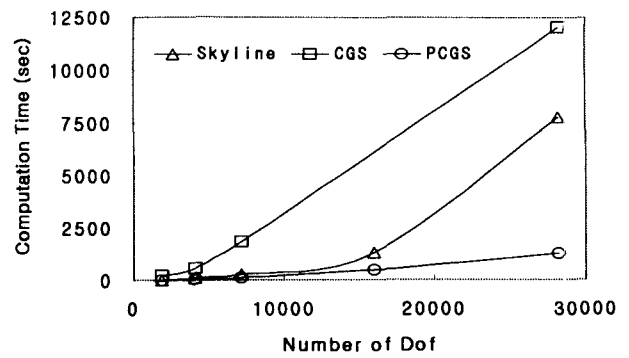
Fig. 4 Time comparison for Kovaszny flow (cubic elements, Re = 40 )
