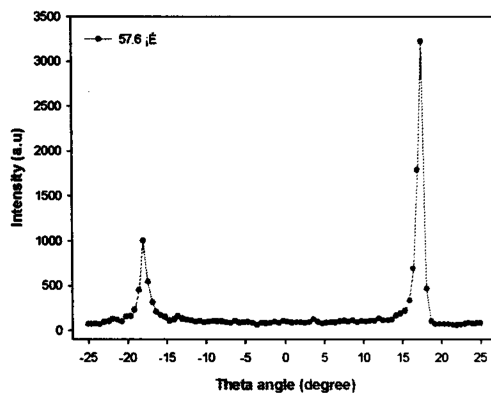
Fig. 4. The theta scan of pure Felix-015/100 at 57.6 °C. The peak positions are symmetric but the intensity of the peaks is not symmetric.
