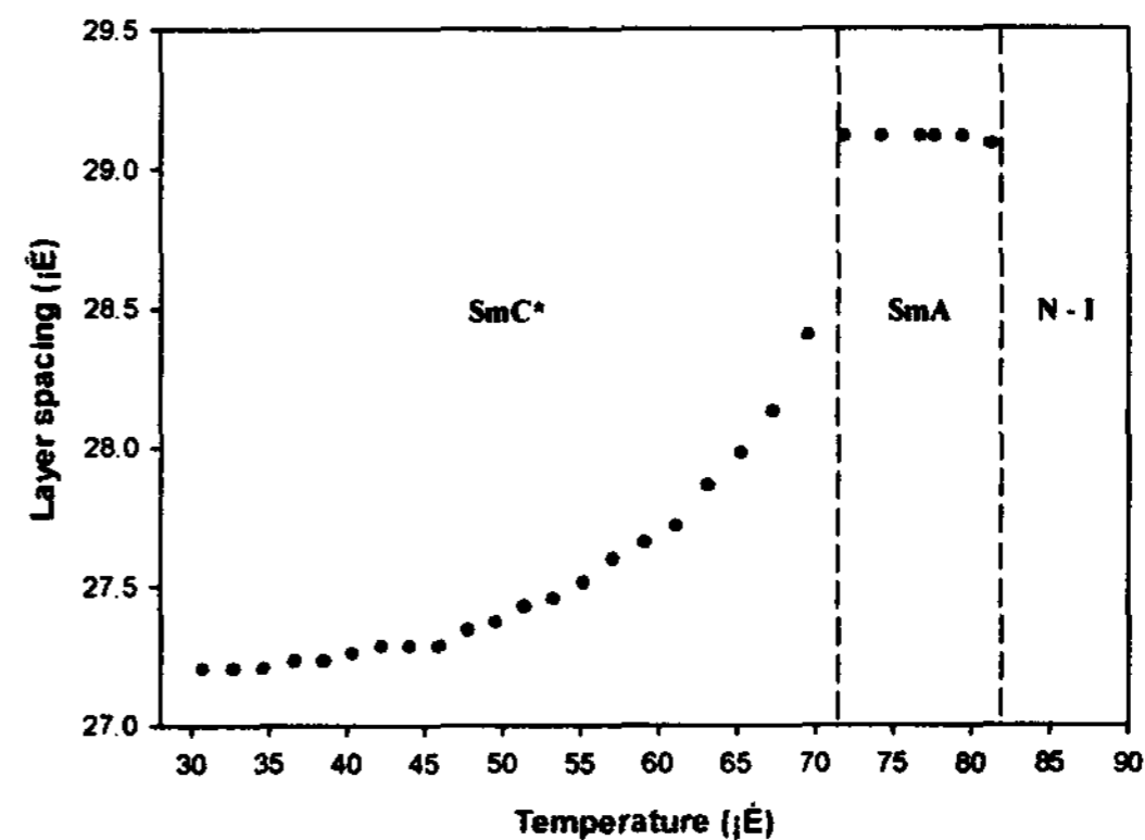
Fig. 2. The layer spacing on temperature for pure Felix-015/100.
