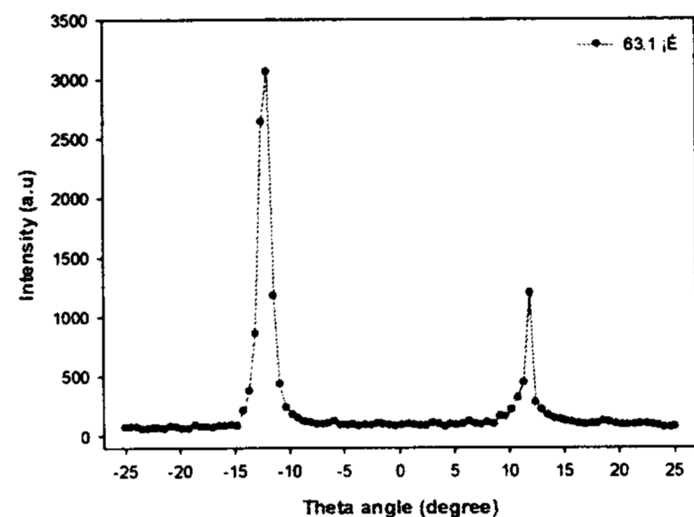
Fig. 6. Theta scan of SSFLC cell made by pure Felix-016/100 FLC at 63.1 °C. The peak positions are symmetric but the intensity of the peaks is not symmetric.
