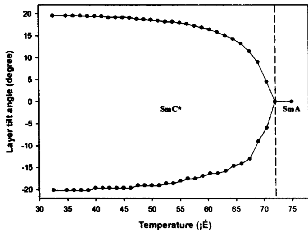
Fig. 3. The temperature dependence of the layer tilt angle for pure Felix-015/100. In Sm C* phase, the layer tilt angle is symmetric.
