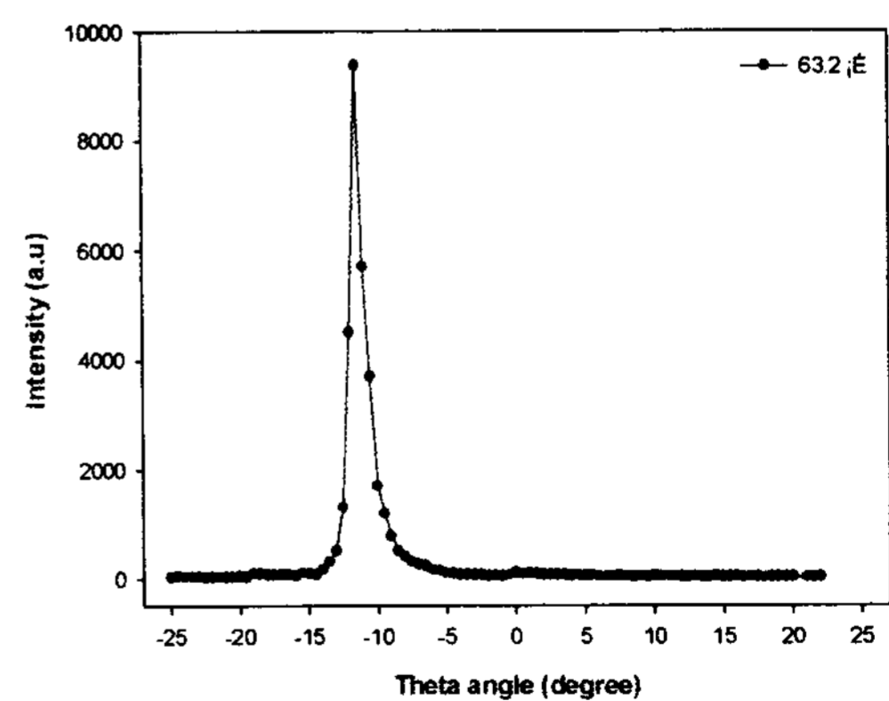
Fig. 7. Theta scan of PSCOF cell made by mixture of Felix-016/100:NOA65=70:30 at 63.2 °C.
