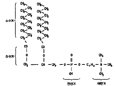
(a) DLPC
