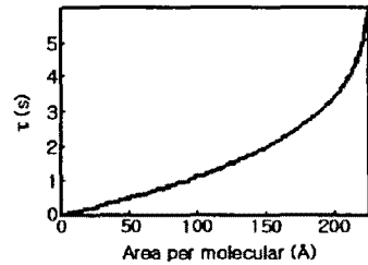
(a) DLPC
