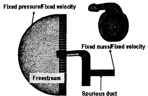
Fig. 4 Grid and boundary conditions.
