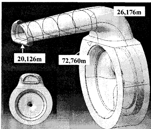
Fig. 3 Cross-section area in the inlet duct.
