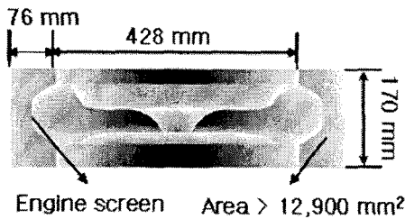
Fig. 2 Cross-section view of plenum chamber.
