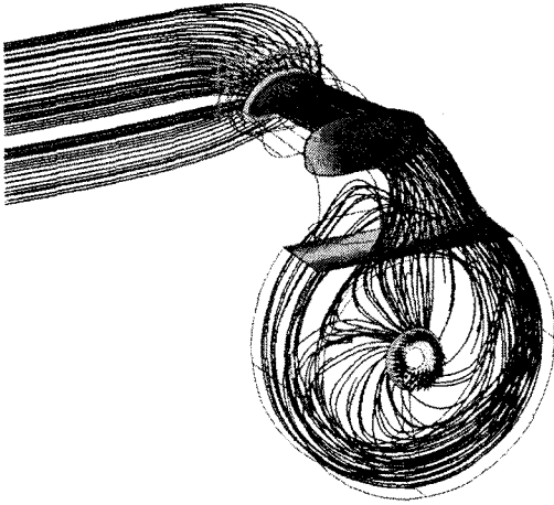
Fig. 7 Streamline distribution in the case of side wind(15m/s).
