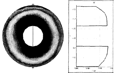
Fig. 10 Total pressure distribution at the compressor inlet.
