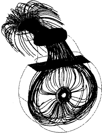
Fig. 9 Streamline distribution in the case of back wind(15m/s).
