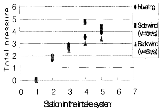
Fig. 8 Total pressure loss in the inlet system with wind direction.
