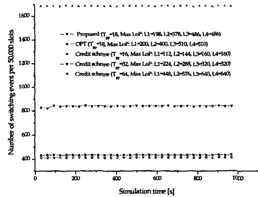
Figure 2: Number of piconet switching events
